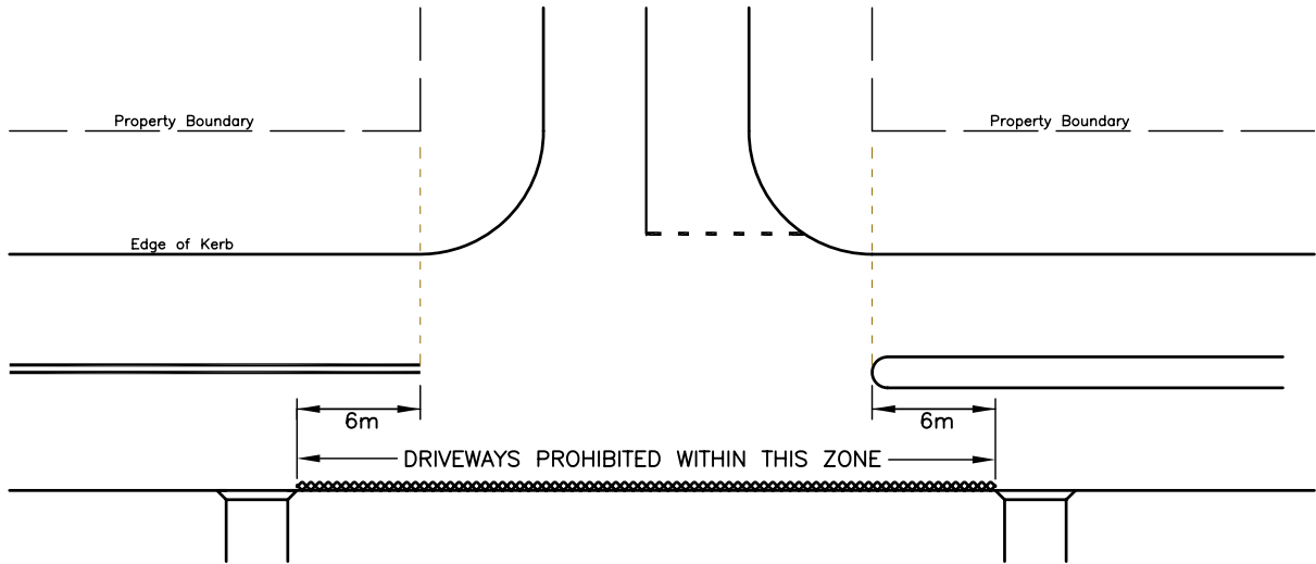
b) Driveway locations in relation to intersections
